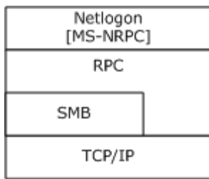
Figure 3: Transport relationships
