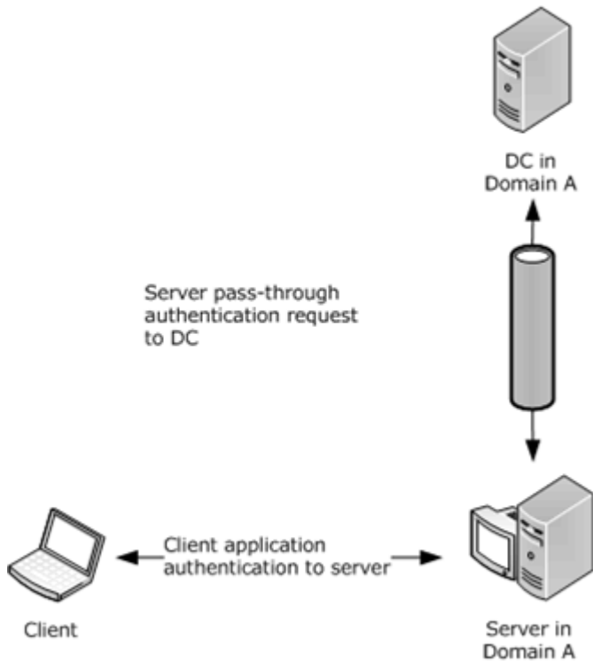
Figure 1: Pass-through authentication
