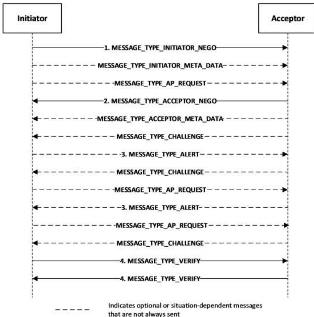
Figure 1: The NEGOTEX message flow
