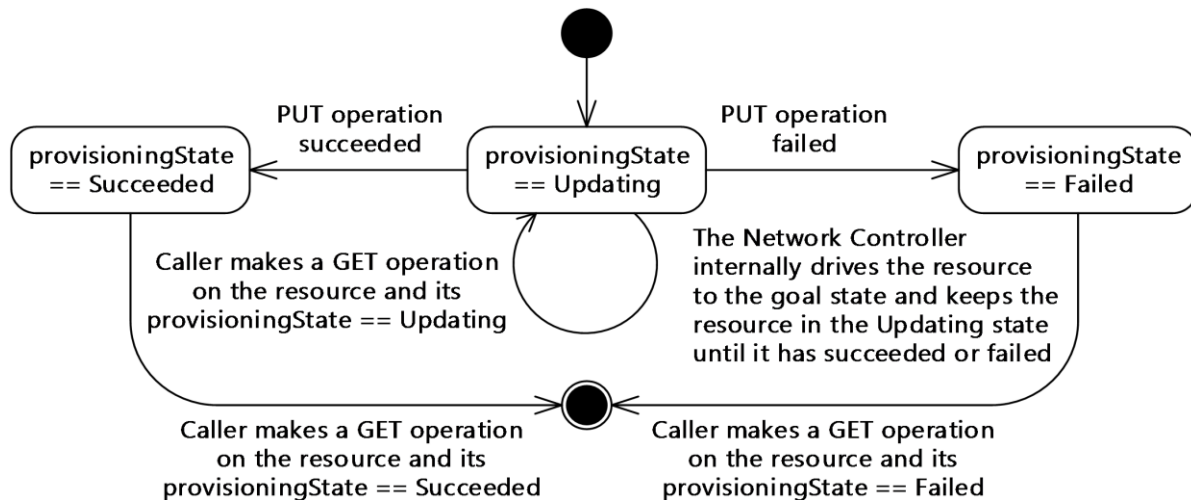
Figure 4: State Diagram s for Asynchronous asynchronous PUT and GET Operations
