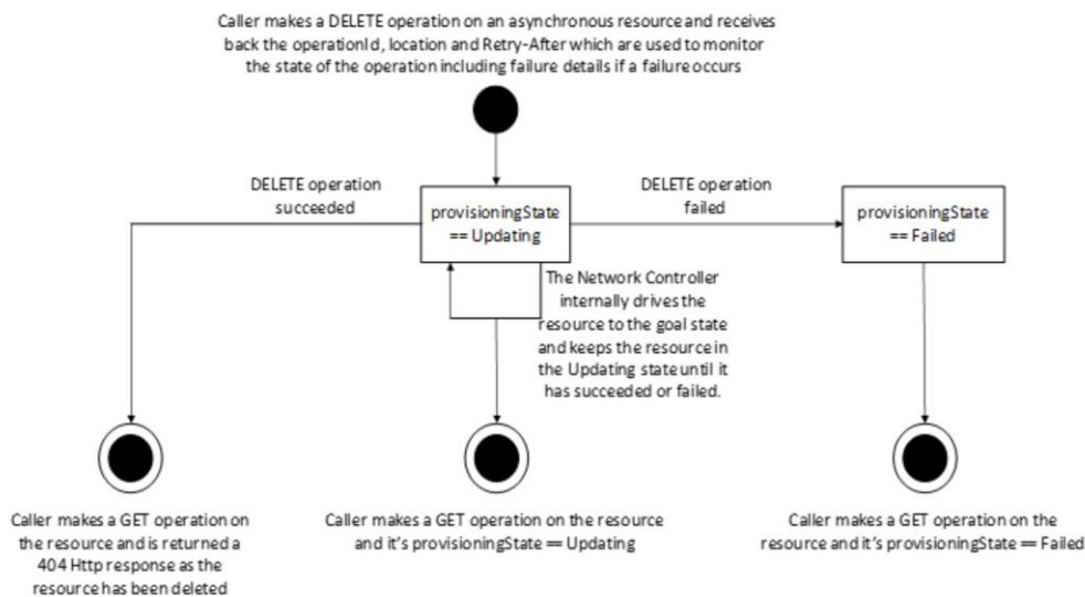
Figure 5: State Diagrams for Asynchronous Delete Operation
