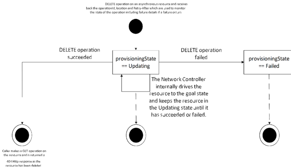
Figure 2: State Diagram for Asynchronous DELETE Operations
