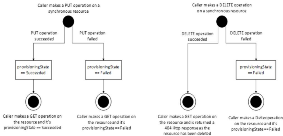
Figure 3: State Diagrams for Synchronous Operations
