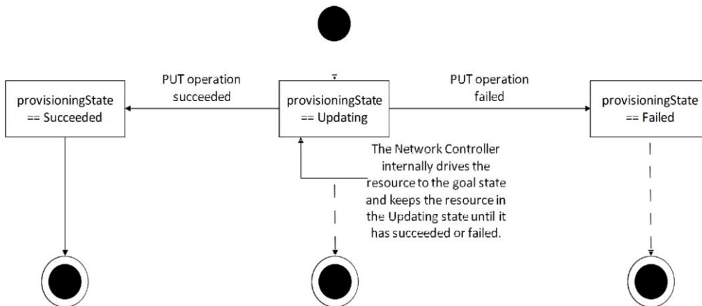
Figure 1: State Diagram for Asynchronous PUT Operations
