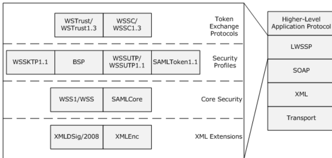
Figure 1: Protocol relationships
