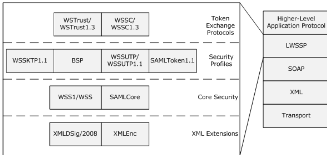
Figure 1: Protocol relationships
