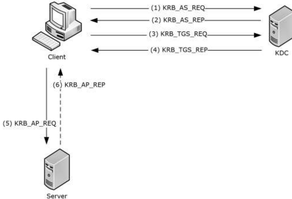
Figure 1: Kerberos V5 Exchanges
