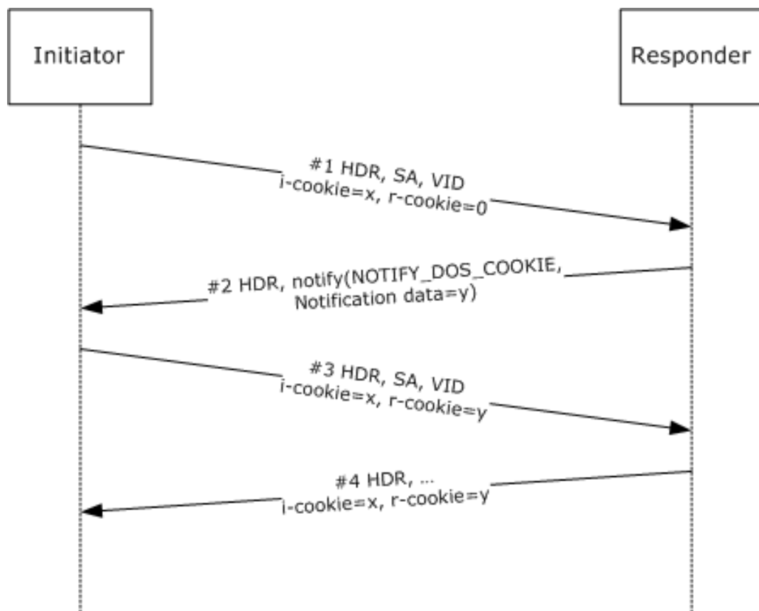
Figure 10: IKE using the DOSDoS Protection extension
