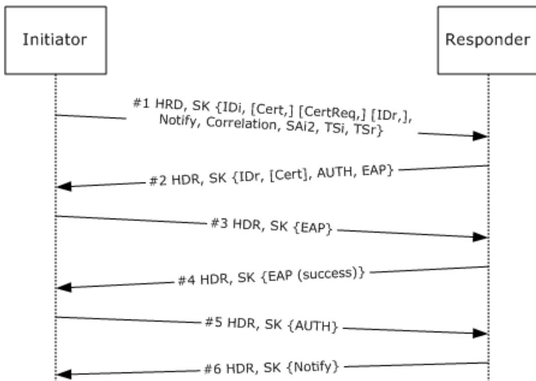
Figure 11: Standard IKEv2 exchange
