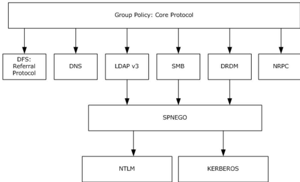
Figure 1: Group Policy: Core Protocol relationship diagram
