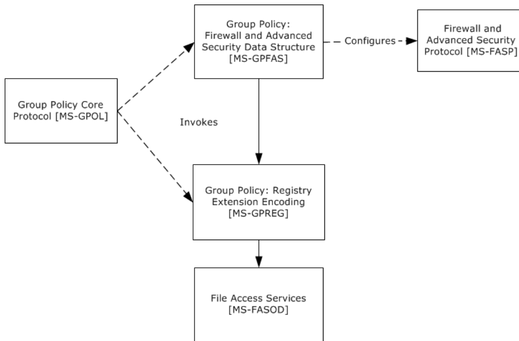
Figure 1: Group Policy: Firewall and Advanced Security Data Structure protocol relationship diagram
