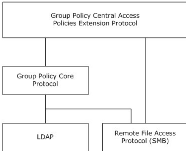
Figure 1: Group Policy: Central Access Policies Extension protocol relationships
