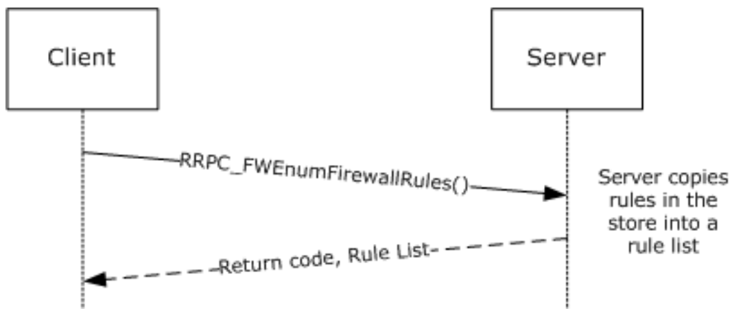
Figure 4: Enumerating firewall rules
