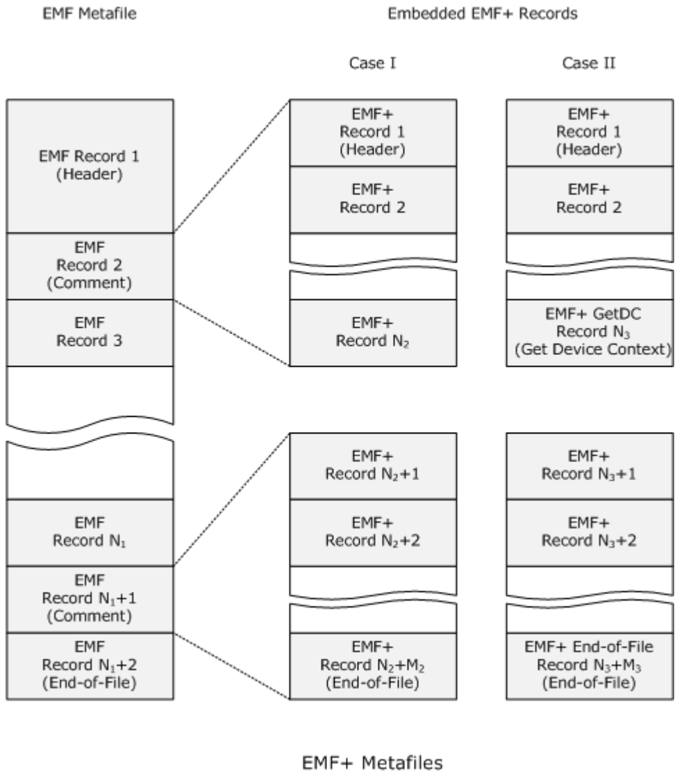
Figure 1: EMF+ metafiles
