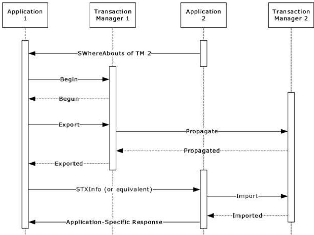
Figure 10: Transaction manager push propagation
