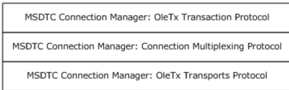
Figure 11: Protocol relationships
