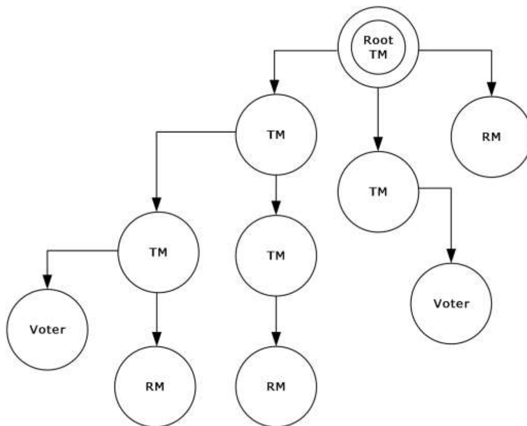
Figure 1: Transaction tree
