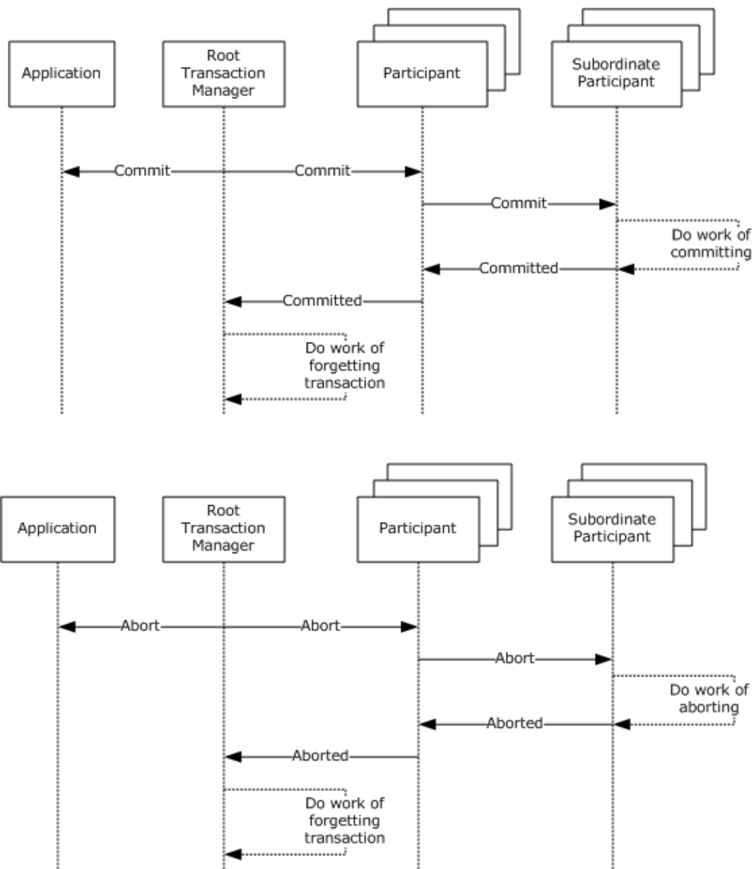
Figure 4: Transaction manager Phase Two flow
