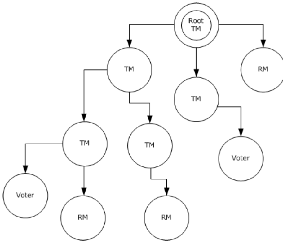
Figure 1: Transaction tree
