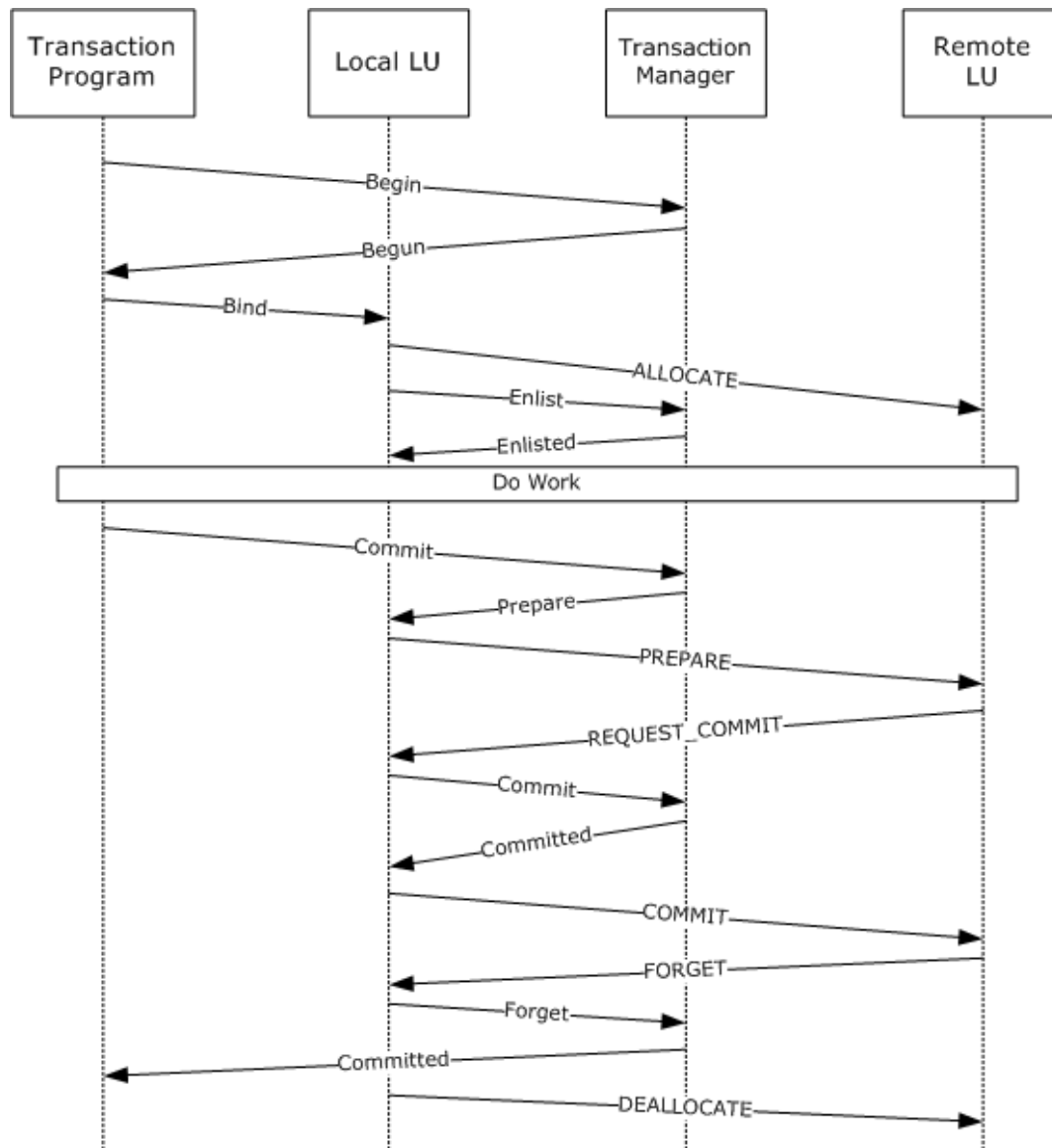
Figure 2: MS-DTCLU enlistment
