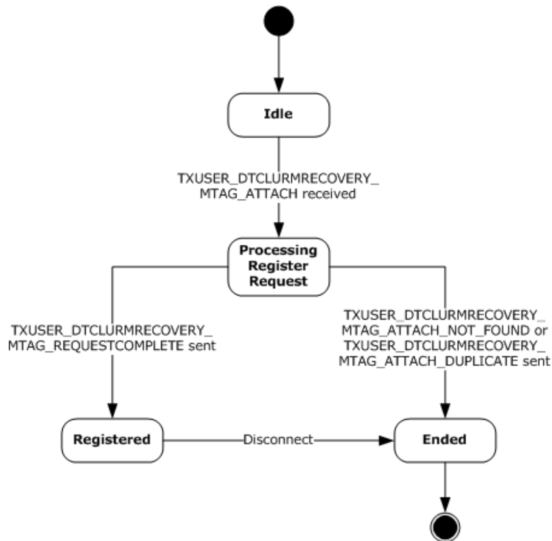
Figure 12: CONNTYPE_TXUSER_DTCLURECOVERY acceptor states
