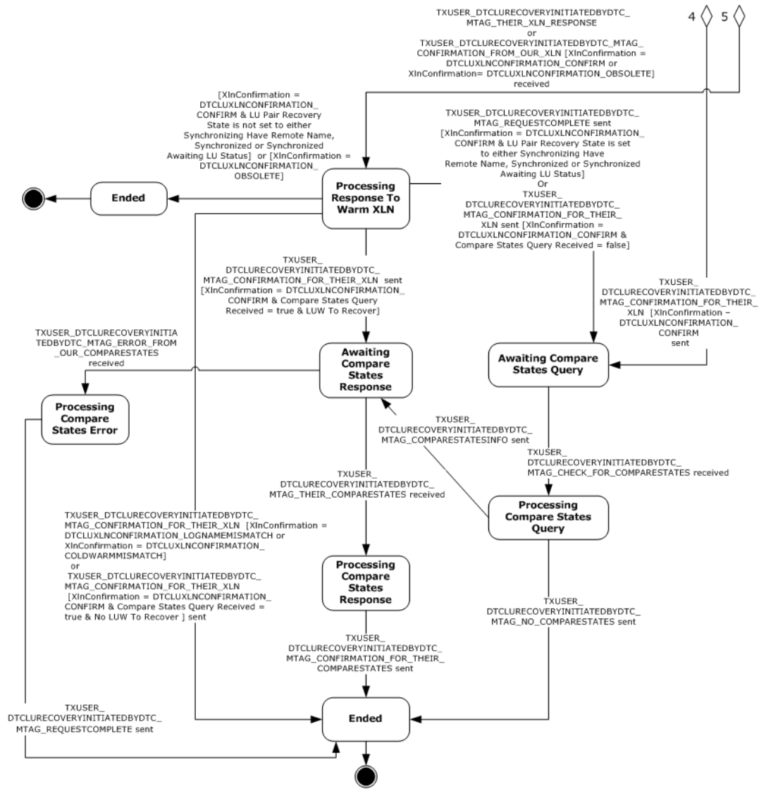
Figure 17: CONNTYPE_TXUSER_DTCLURECOVERYINITIATEDBYDTC, Part 4
