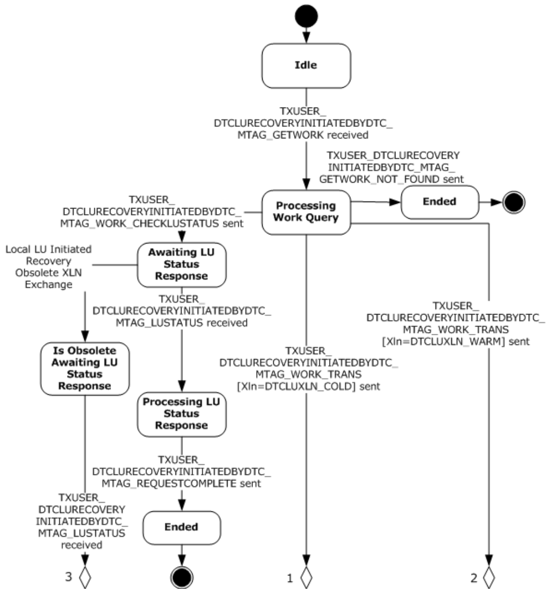
Figure 14: CONNTYPE_TXUSER_DTCLURECOVERYINITIATEDBYDTC, Part 1
