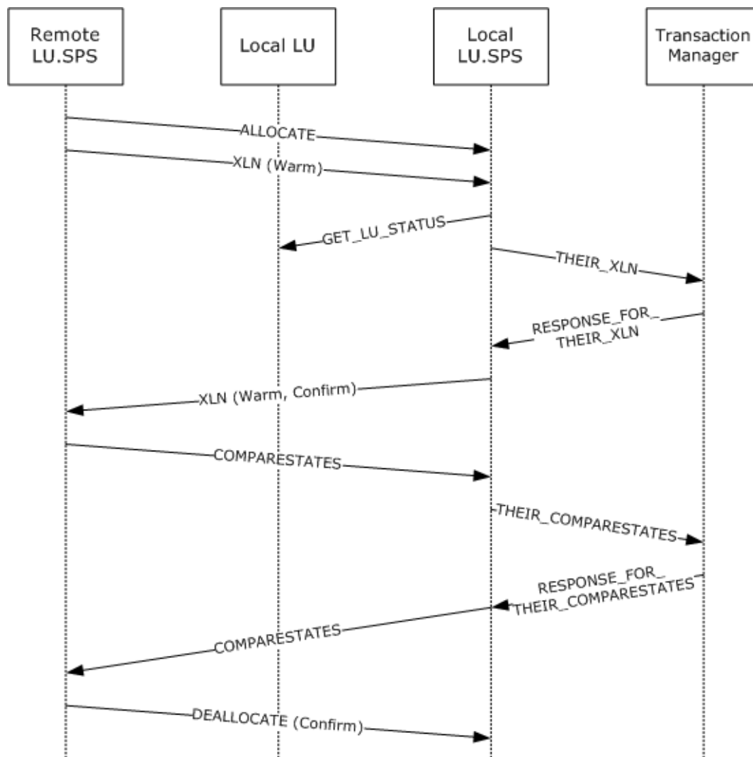
Figure 3: MS-DTCLU recovery
