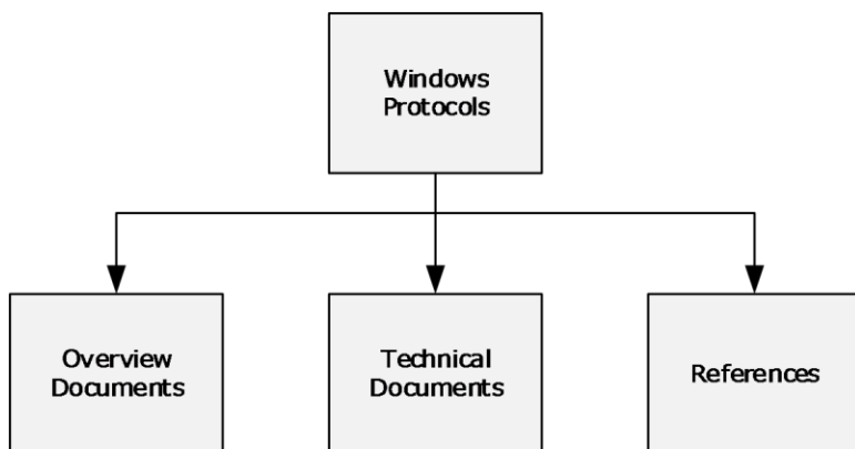
Figure 5: Windows Protocols
