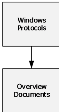
Figure 7: Overview documents
