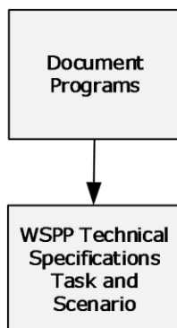
Figure 4: Document programs
