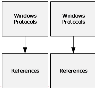
Figure 14: Reference documents
