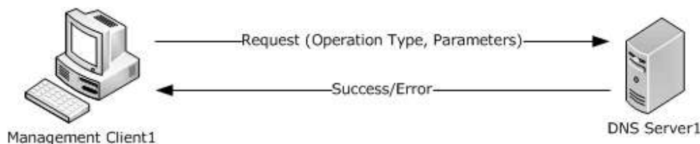
Figure 1: DNS Server Management Protocol
