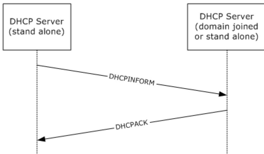
Figure 3: DHCPv4 Server Authorization messages
