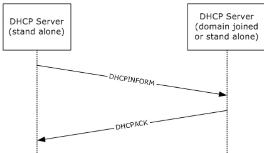
Figure 3: DHCPv4 Server Authorization messages
