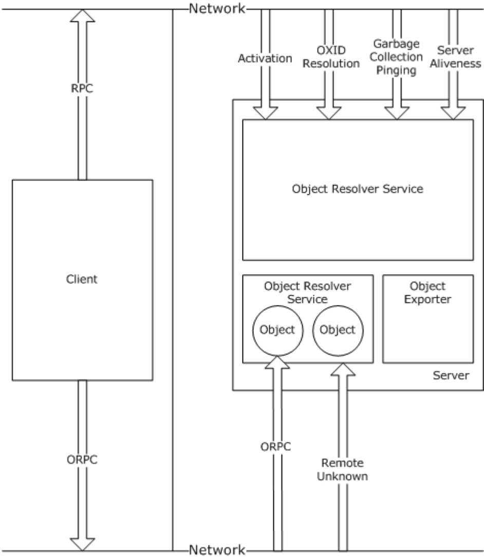
Figure 2: DCOM protocol overview
