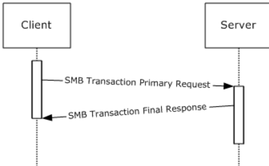
Figure 3: Simple Transaction
