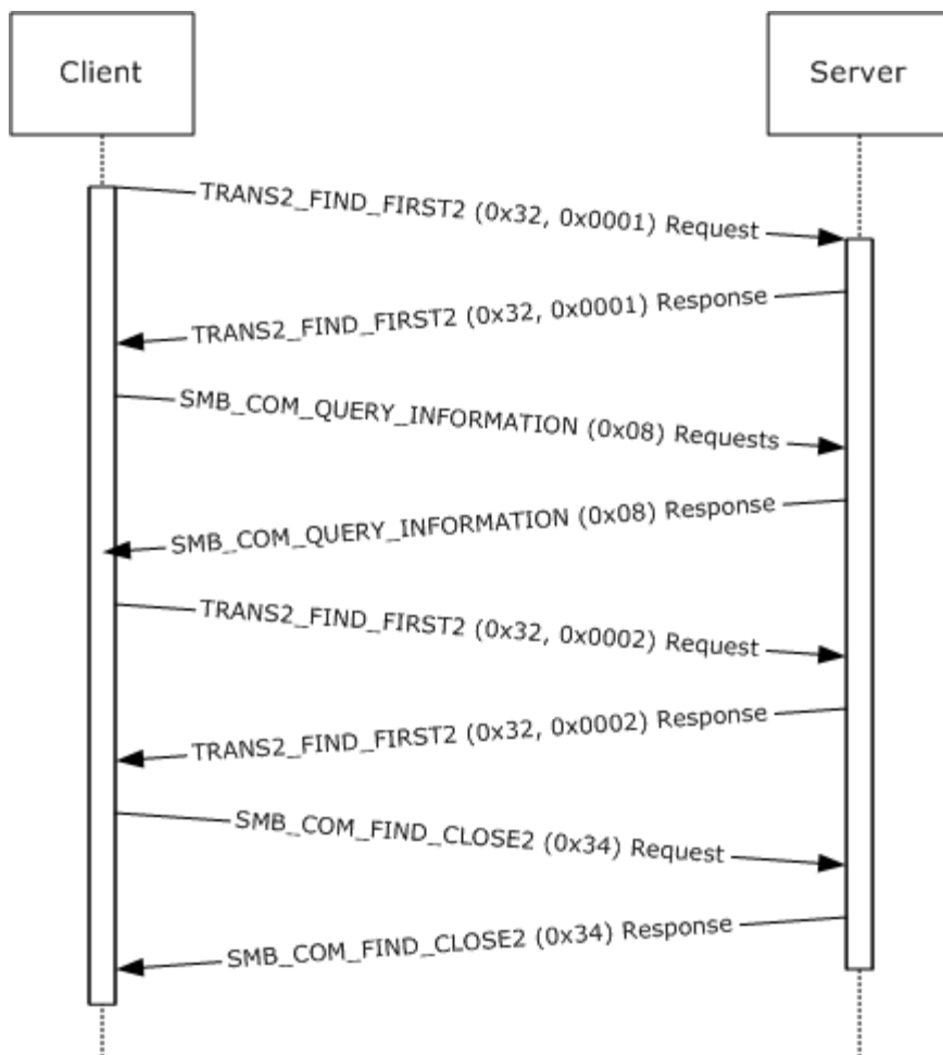
Figure 13: Getting file attributes information
