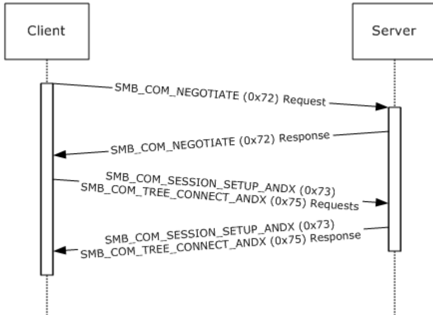
Figure 10: Protocol negotiation and connecting to a share
