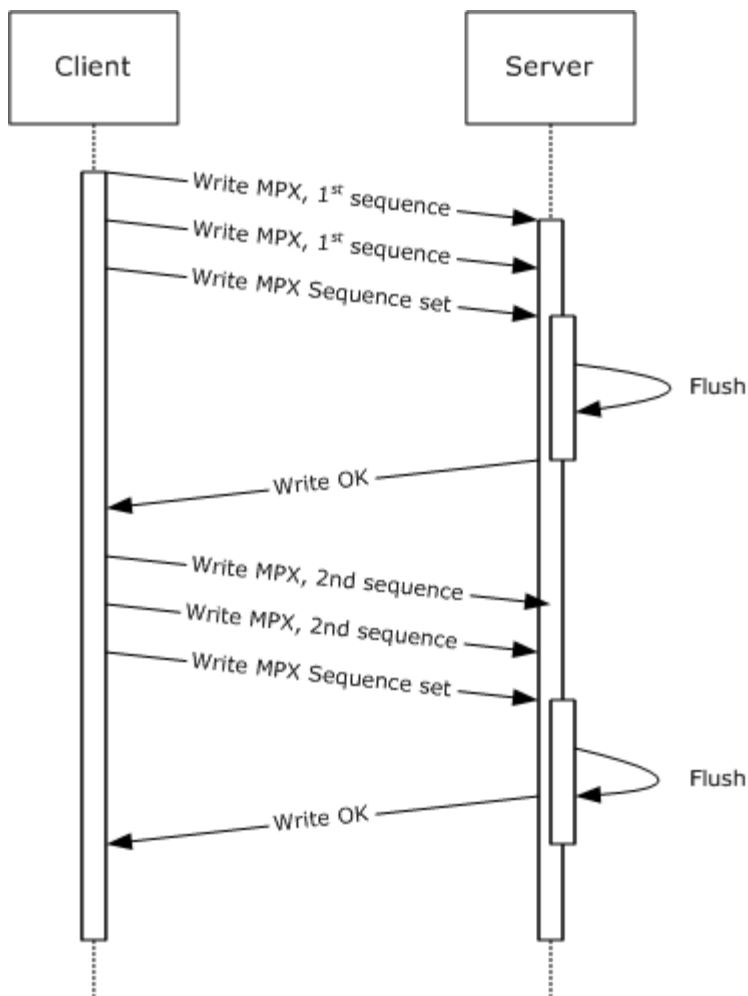
Figure 9: Multiplexed Write request/response message flow
