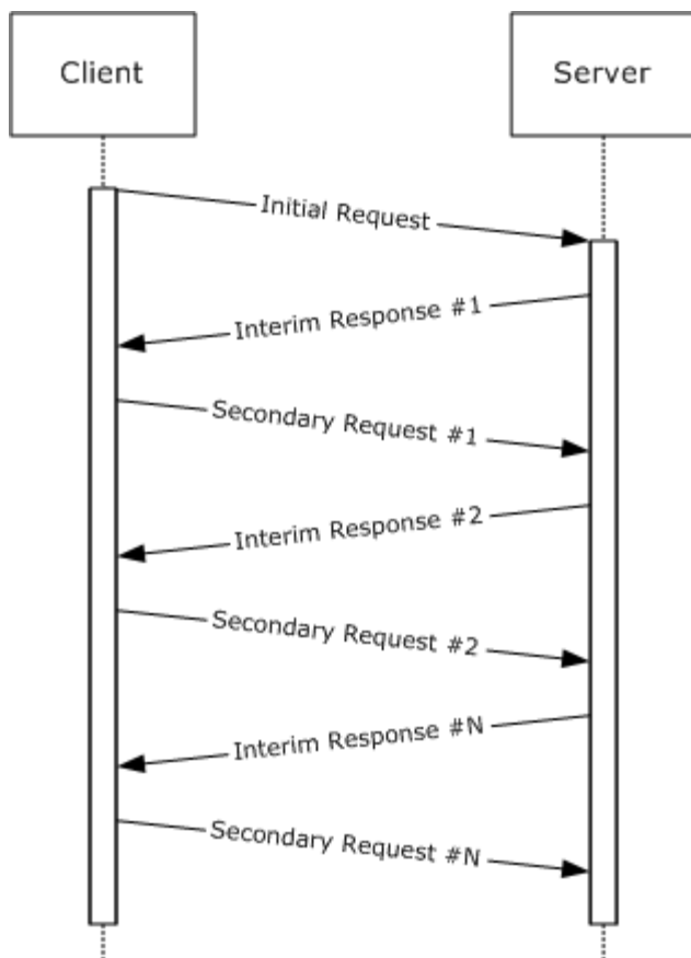
Figure 1: CIFS transaction messages over connectionless transport
