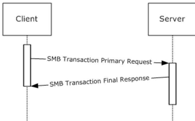
Figure 3: Simple Transaction
