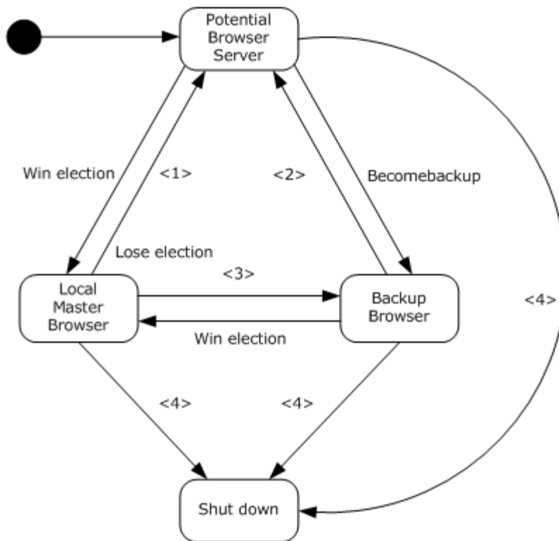
Figure 2: Browser server state machine
