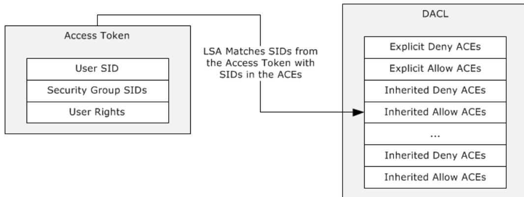
Figure 5: Evaluation process for access tokens against a DACL
