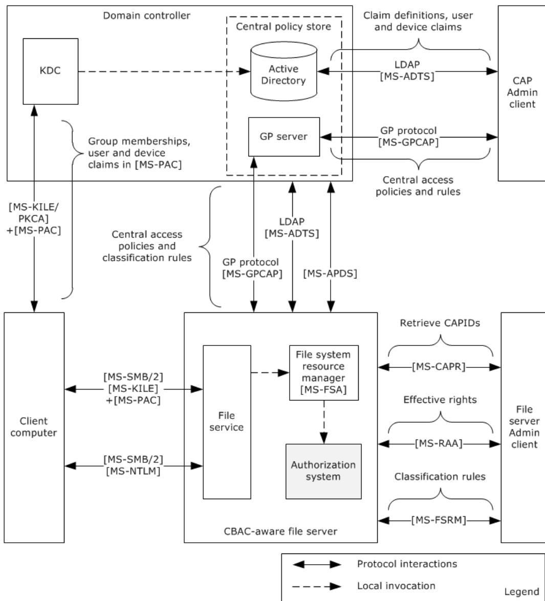
Figure 10: CBAC architecture
