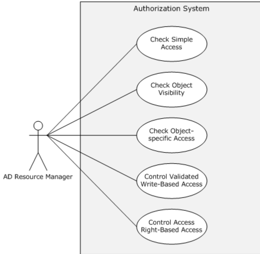
Figure 15: Active Directory authorization use cases
