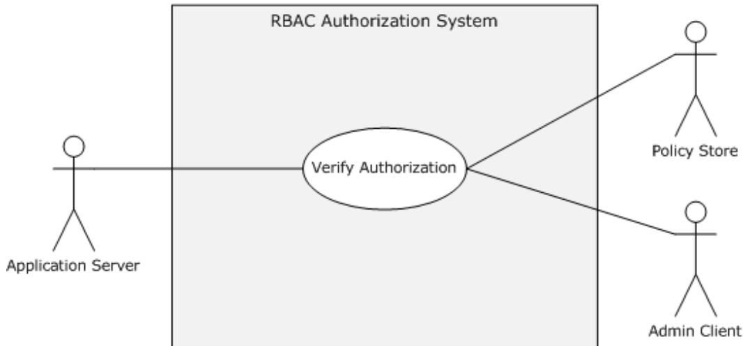
Figure 17: Verify Authorization use case
