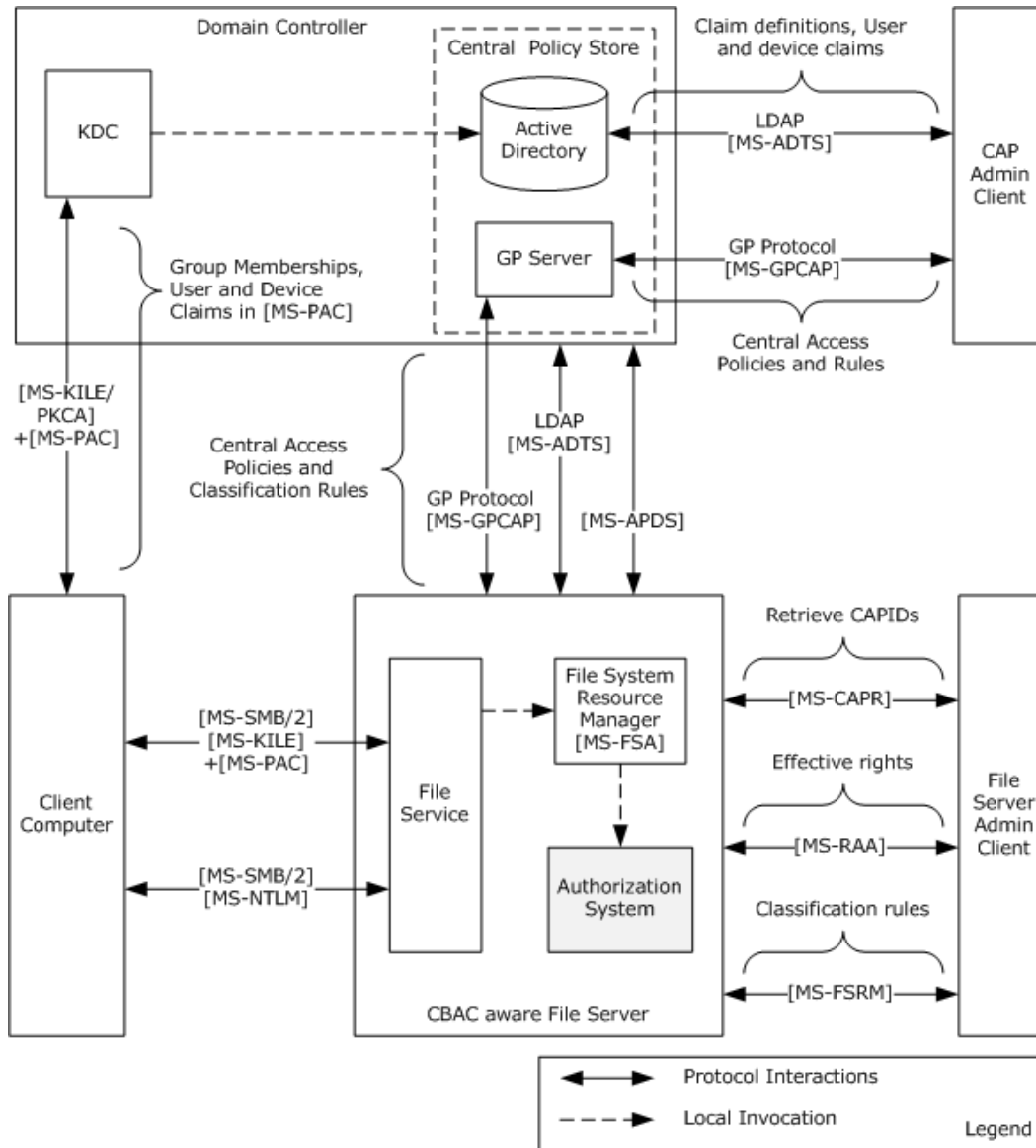
Figure 10: CBAC architecture
