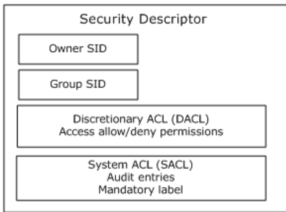
Figure 4: Abstract representation of security descriptor
