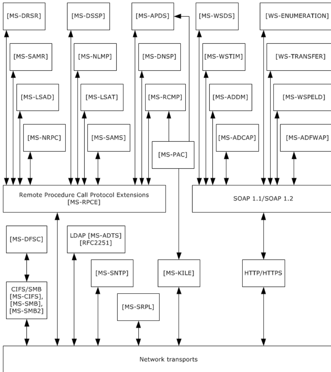
Figure 4: Protocol relationships
