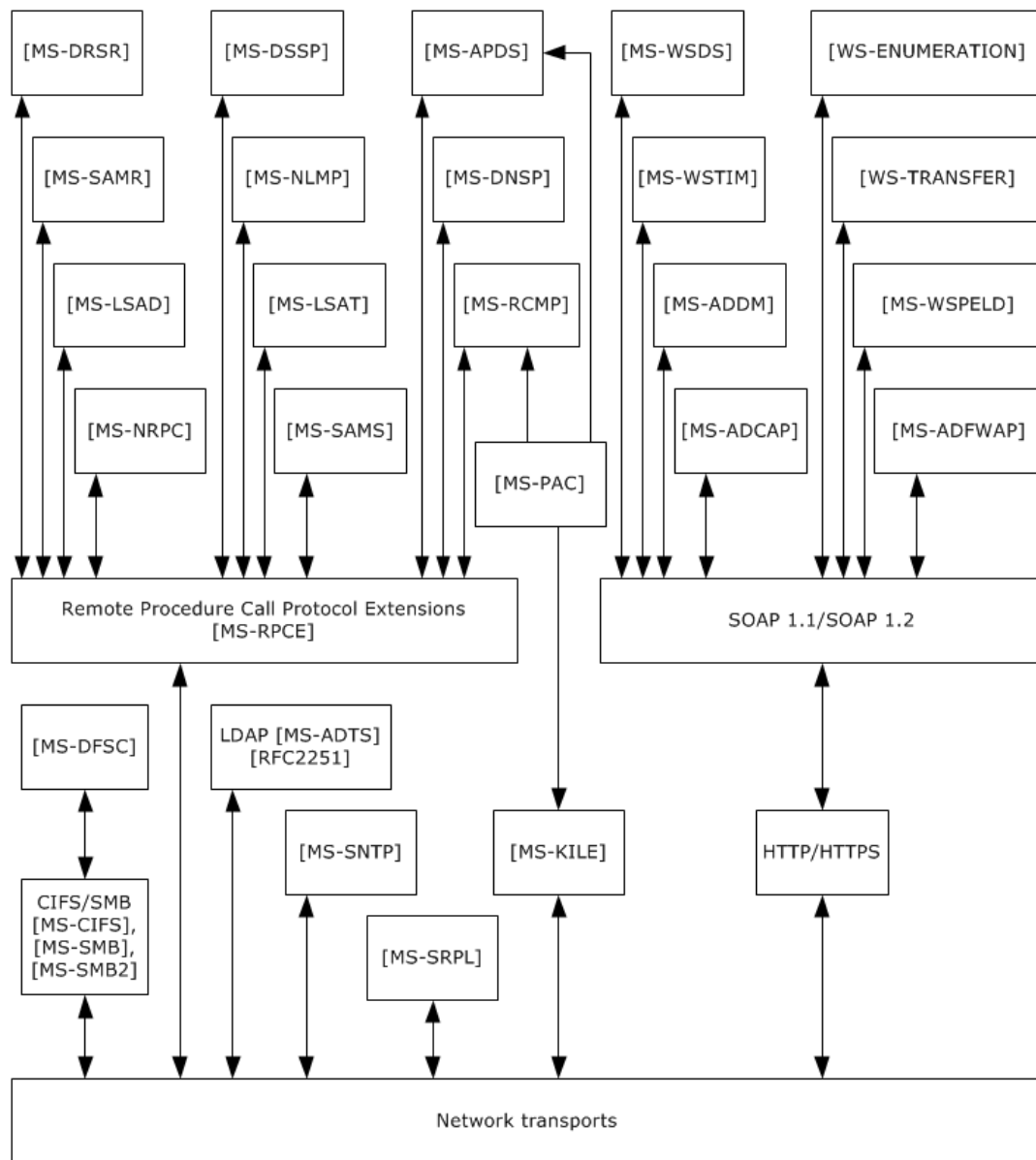
Figure 4: Protocol relationships
