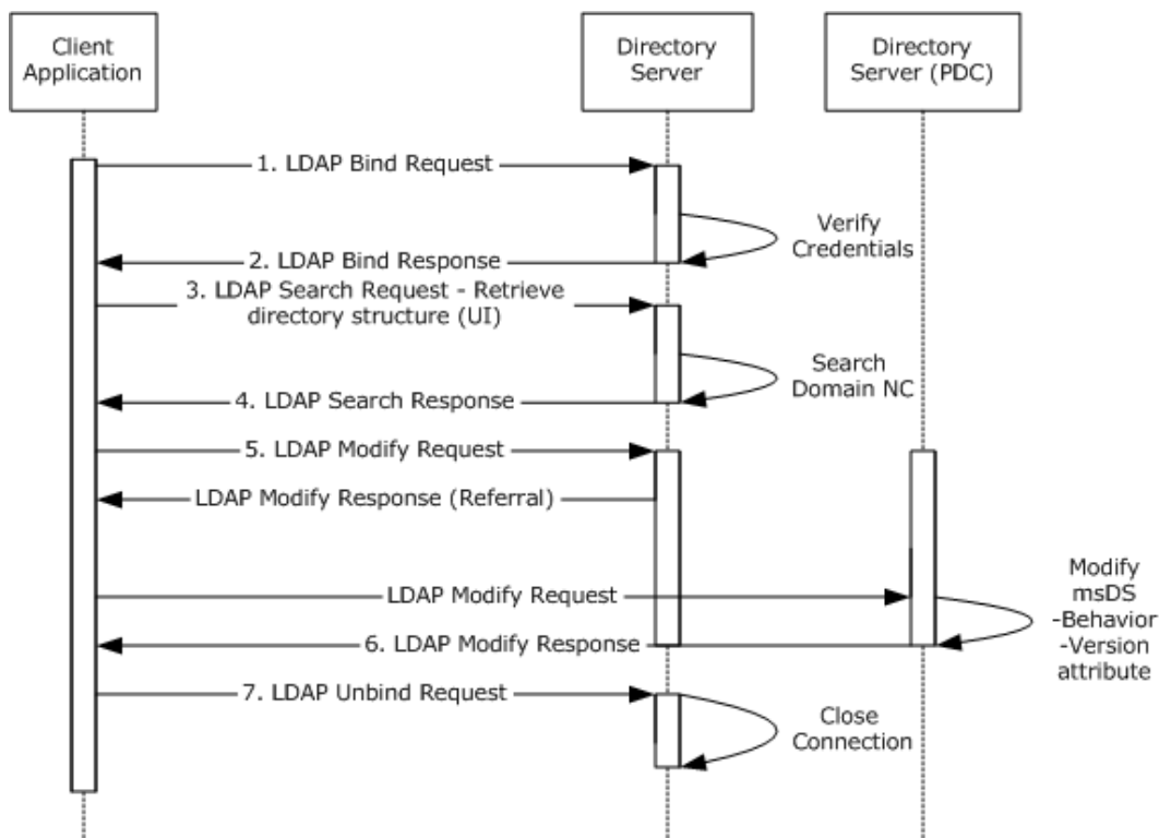
Figure 64: Message flow to raise the domain functional level
