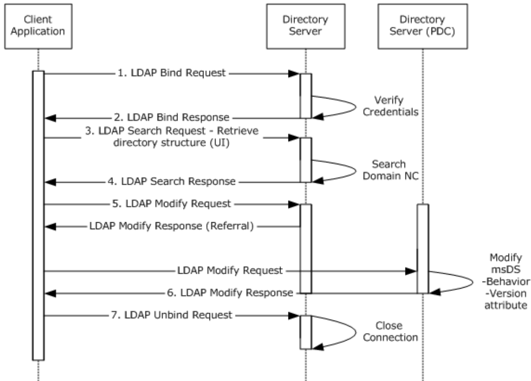
Figure 64: Message flow to raise the domain functional level
