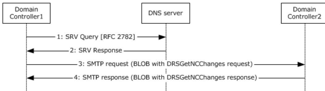
Figure 67: Message flow to replicate changes to a GC or a partial replica
