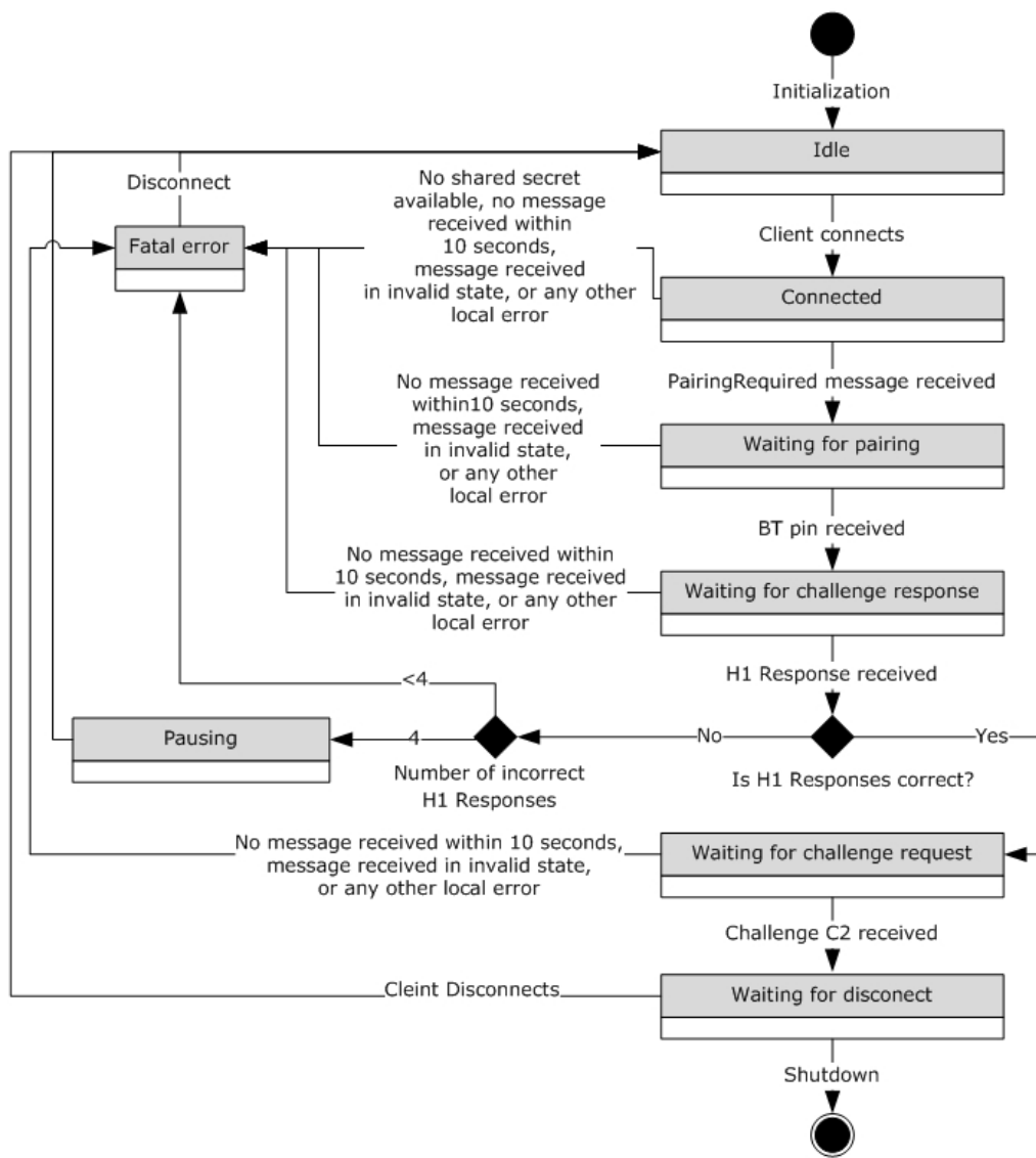
Figure 3: Server state diagram
