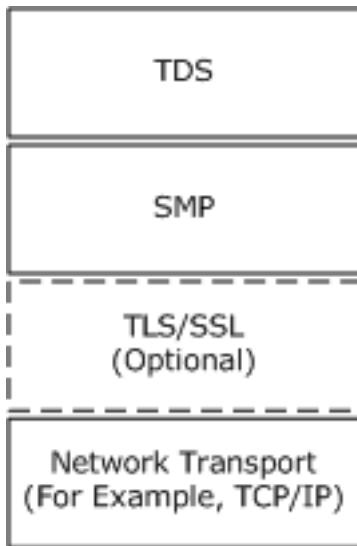
Figure 2: Protocol relationship
