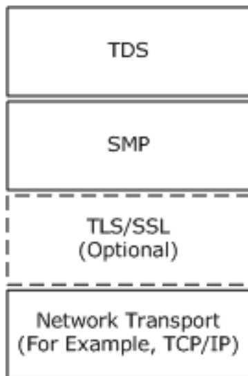
Figure 2: Protocol relationship
