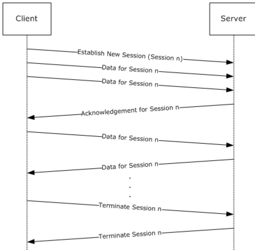
Figure 1: Example of a communication flow in SMP
