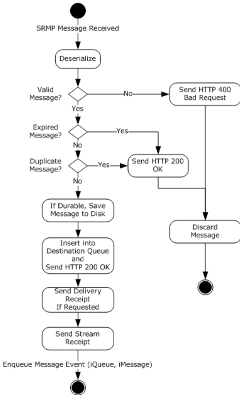
Figure 7: Stream message state receiver
