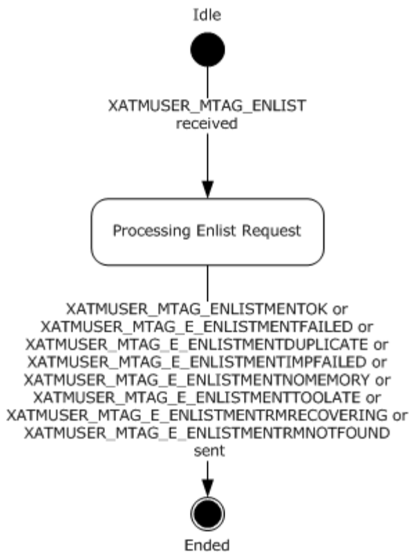
Figure 29: CONNTYPE_XATM_ENLIST acceptor states
