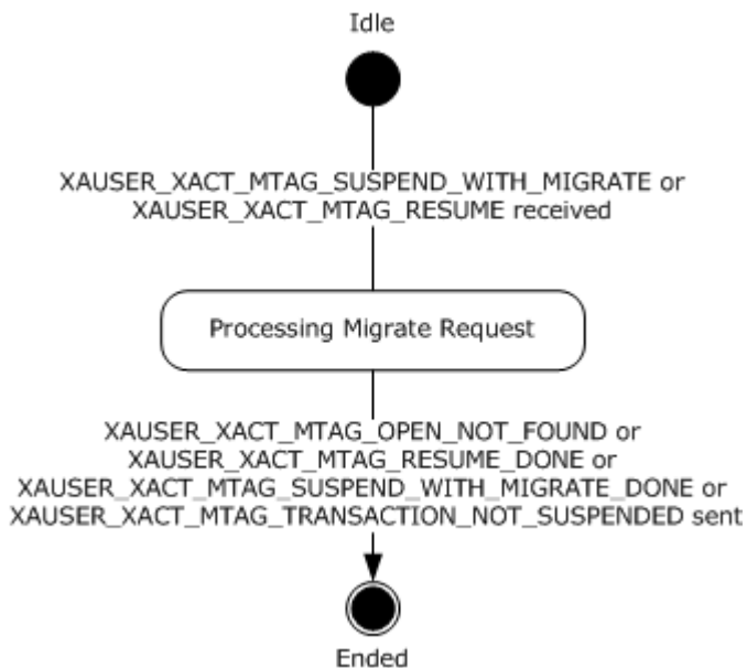
Figure 15: CONNTYPE_XAUSER_XACT_MIGRATE acceptor states
