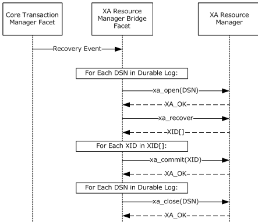
Figure 7: XA Resource Manager Transaction recovery
