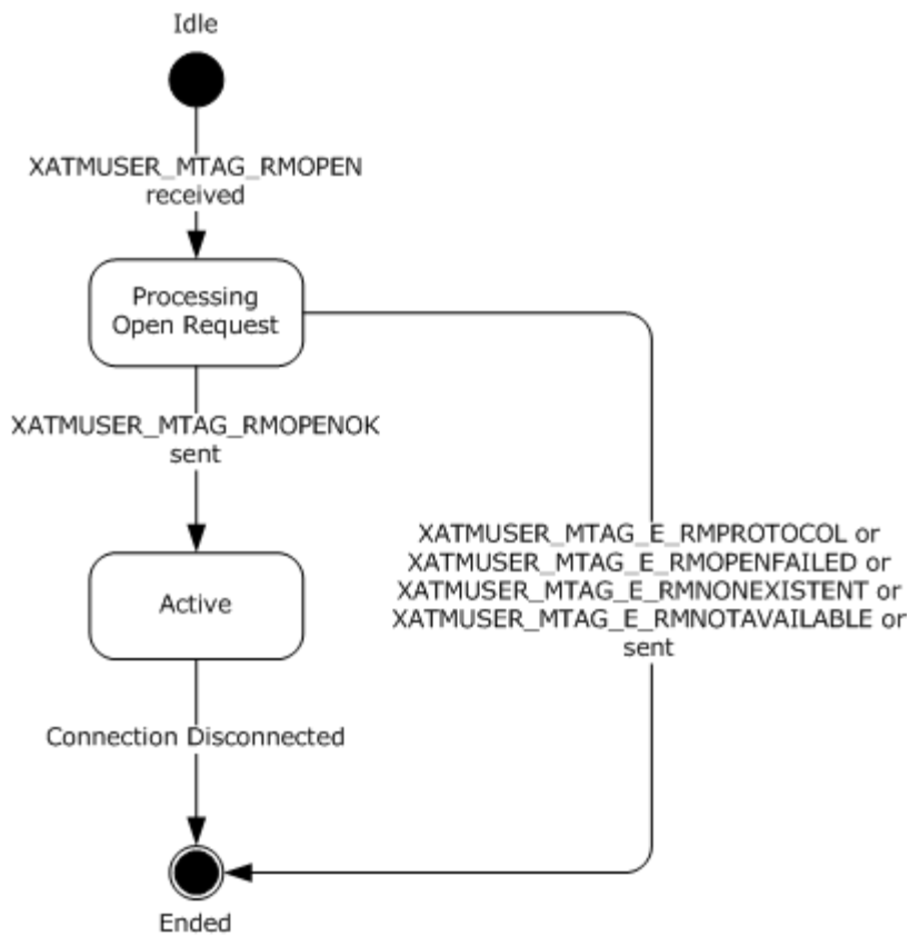
Figure 27: CONNTYPE_XATM_OPEN acceptor states
