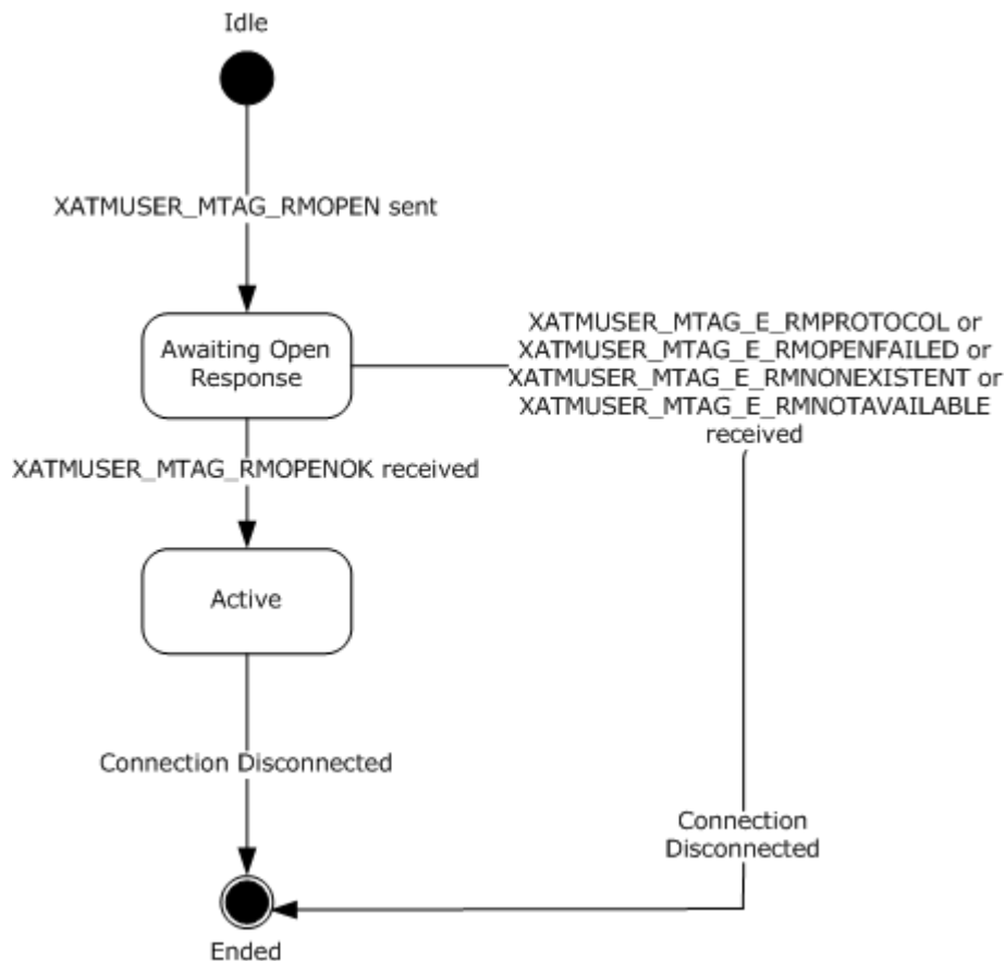
Figure 30: CONNTYPE_XATM_OPEN initiator states
