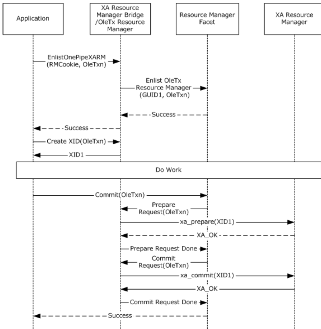
Figure 11: One-pipe XA Resource Manager transaction enlistment and completion
