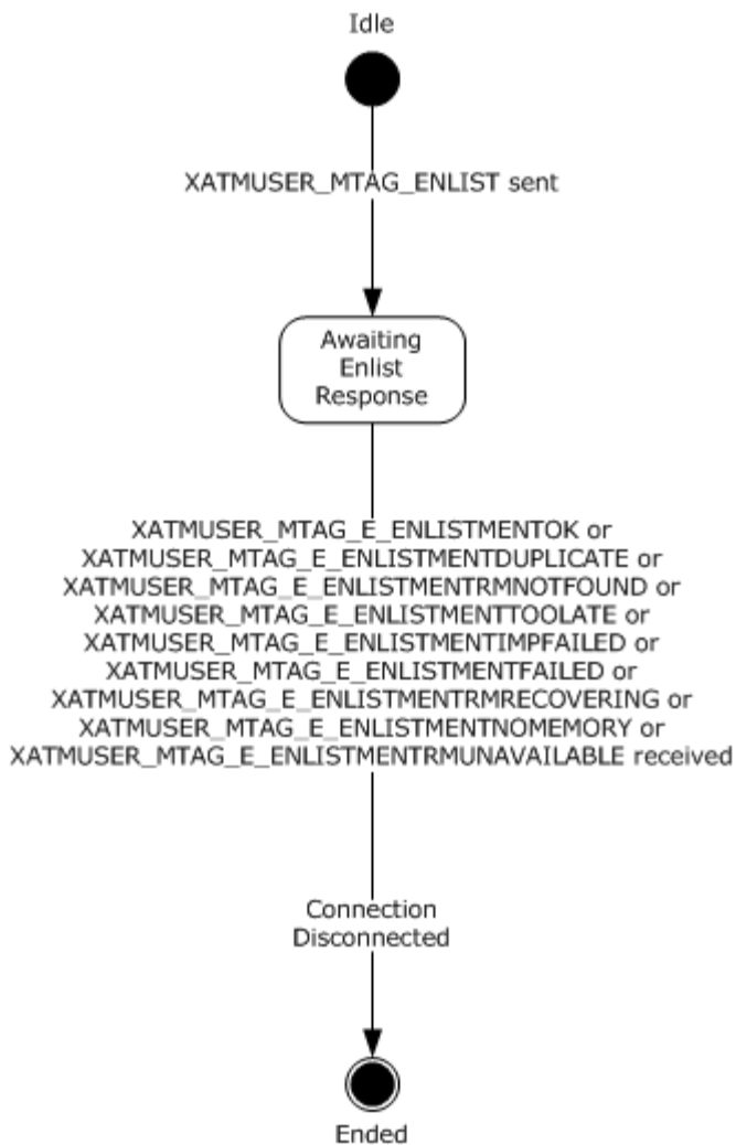
Figure 32: CONNTYPE_XATM_ENLIST initiator states
