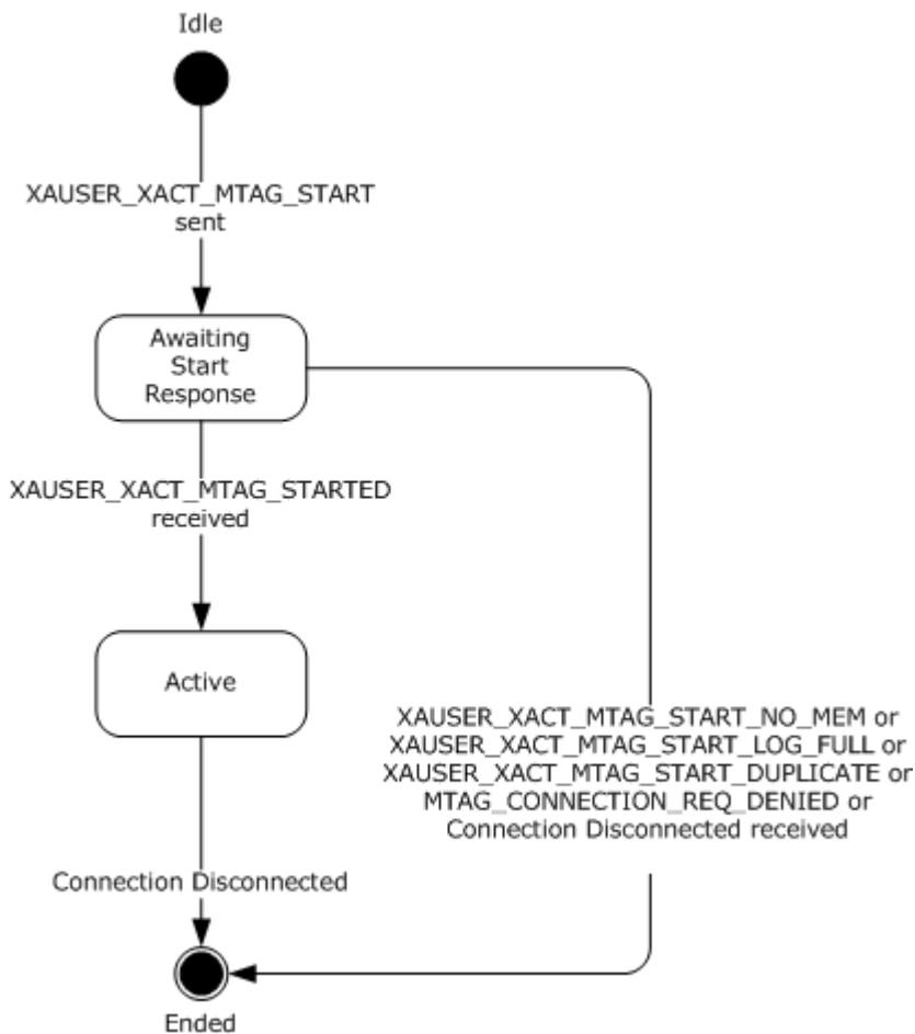
Figure 24: CONNTYPE_XAUSER_XACT_BRANCH_START initiator states
