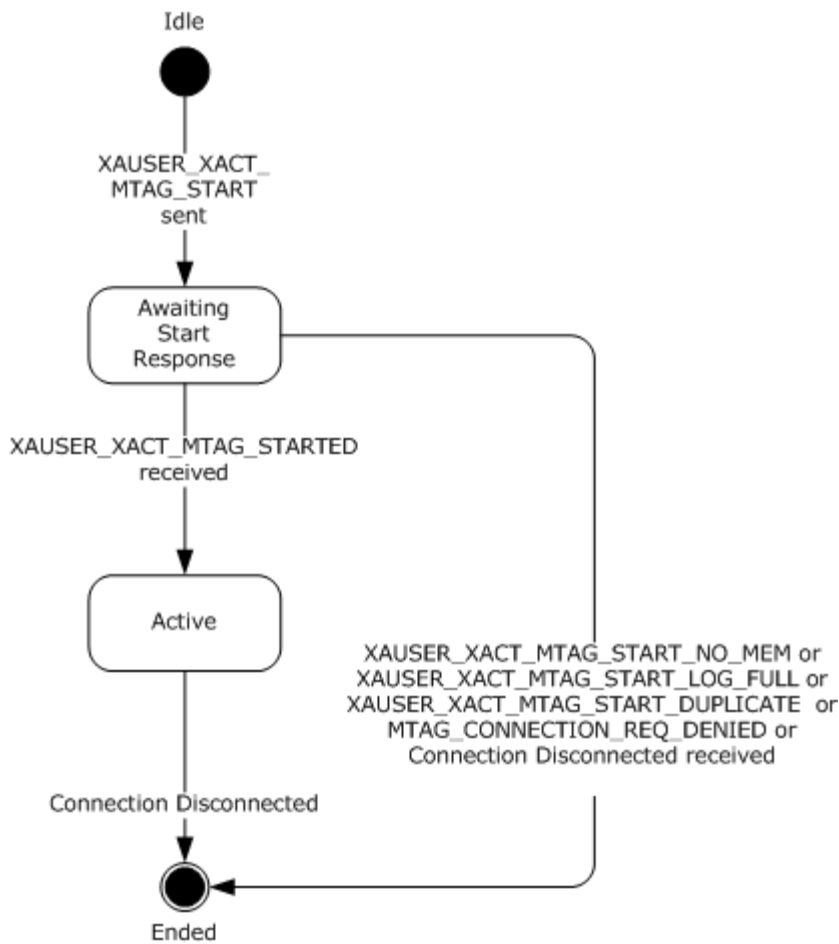
Figure 21: CONNTYPE_XAUSER_XACT_START initiator states
