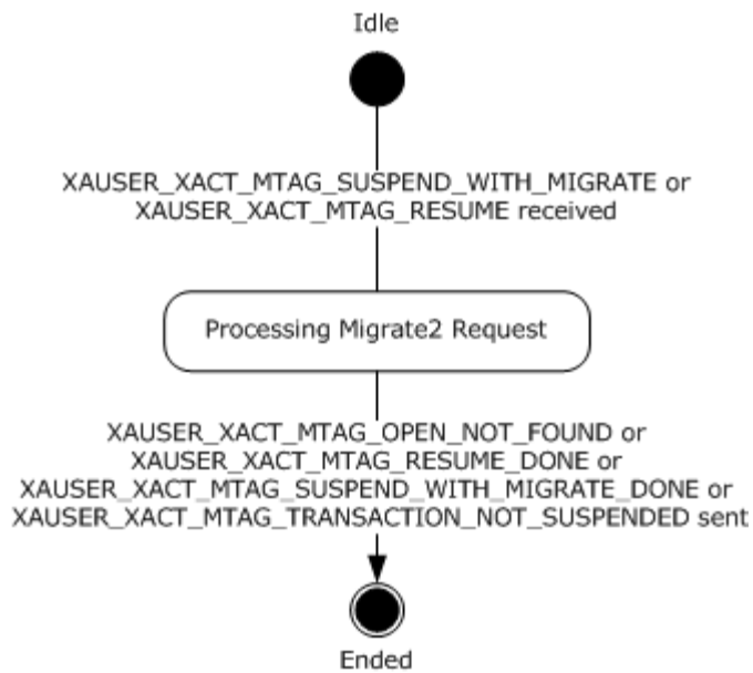
Figure 18: CONNTYPE_XAUSER_XACT_MIGRATE2 acceptor states
